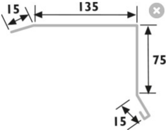
VERGE TRIM
