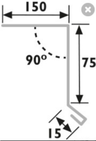
EAVE FLASHING
