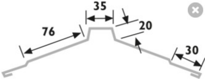
RIDGE CAP FOR TRAPEZOIDAL PROFILES
